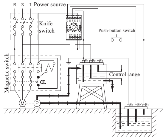
Water-supply running with prevention of idle running of pump.
