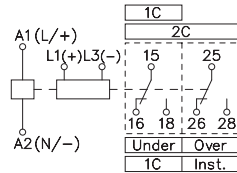
DC Type
