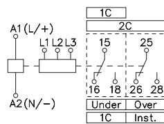
3 Phase 3 Wire
