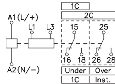
Single Phase
