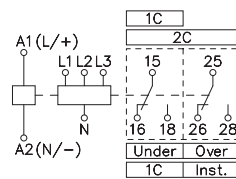
3 Phase 4 Wire
